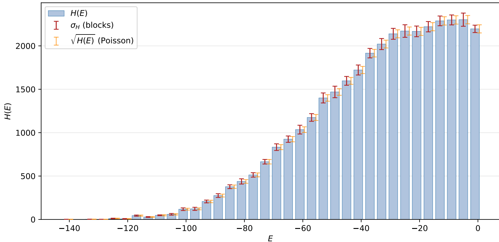
Energy histogram H(E) , L = 16 , \beta_c 16 blocks of 4096 sweeps
