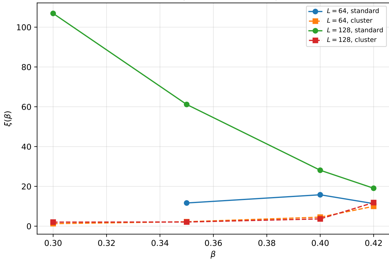
Correlation length vs. inverse temperature
