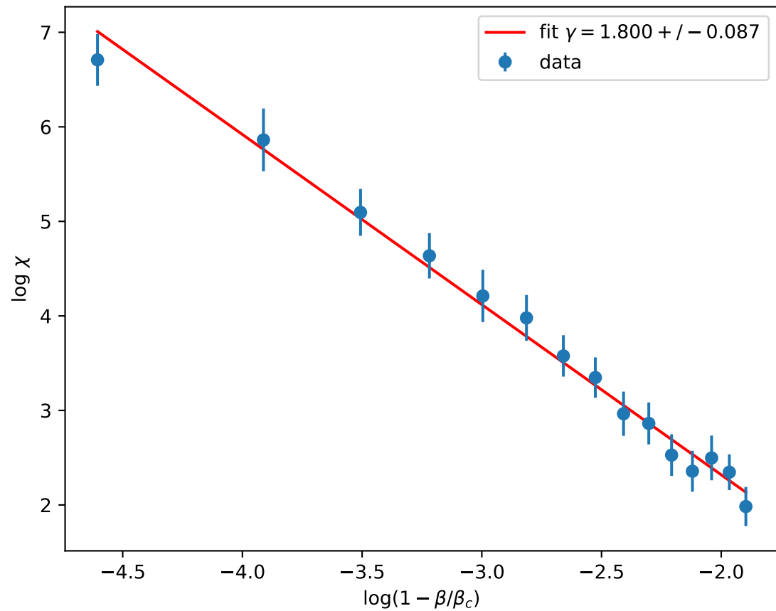
Log-log: slope = -\gamma
