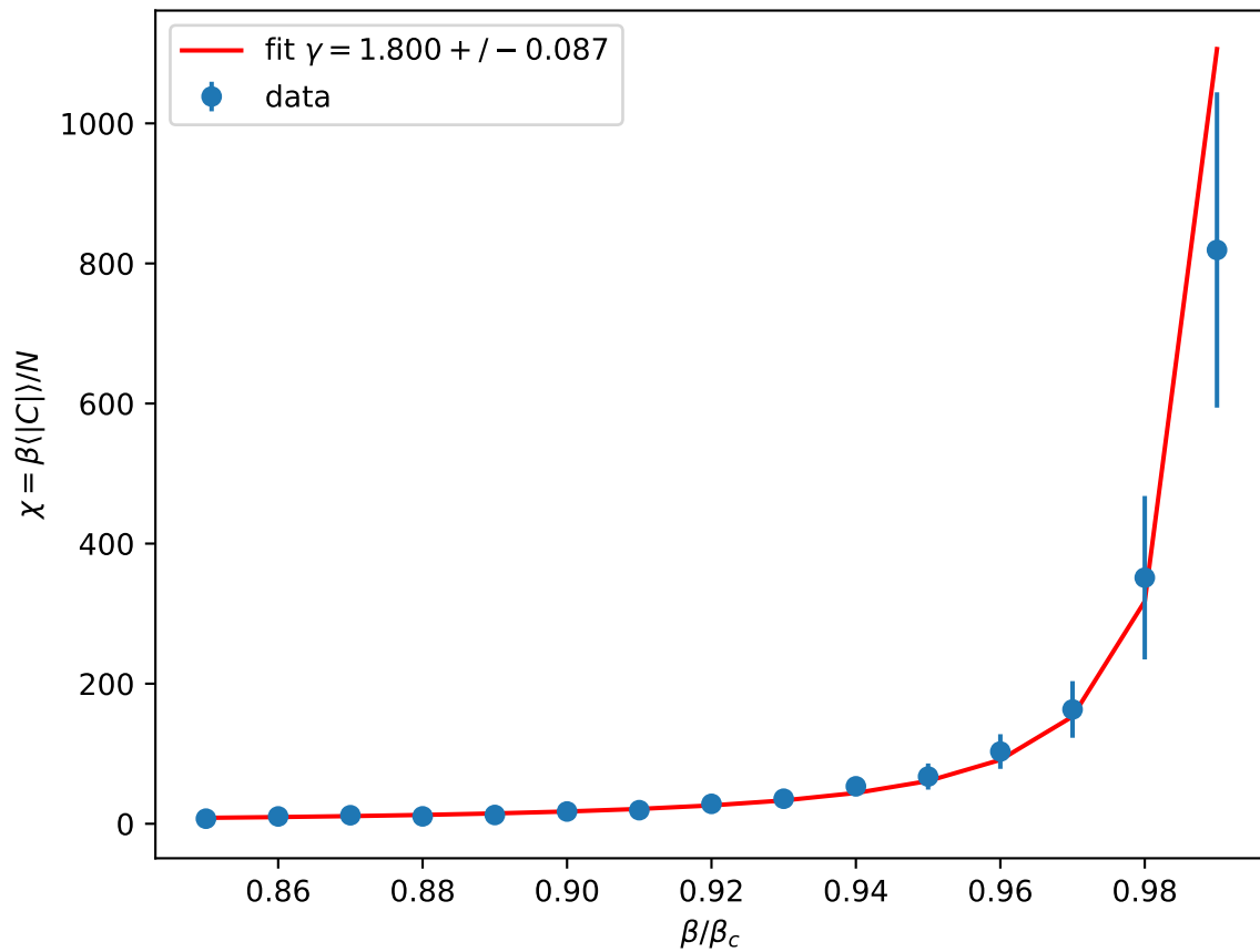
Susceptibility vs. \beta
