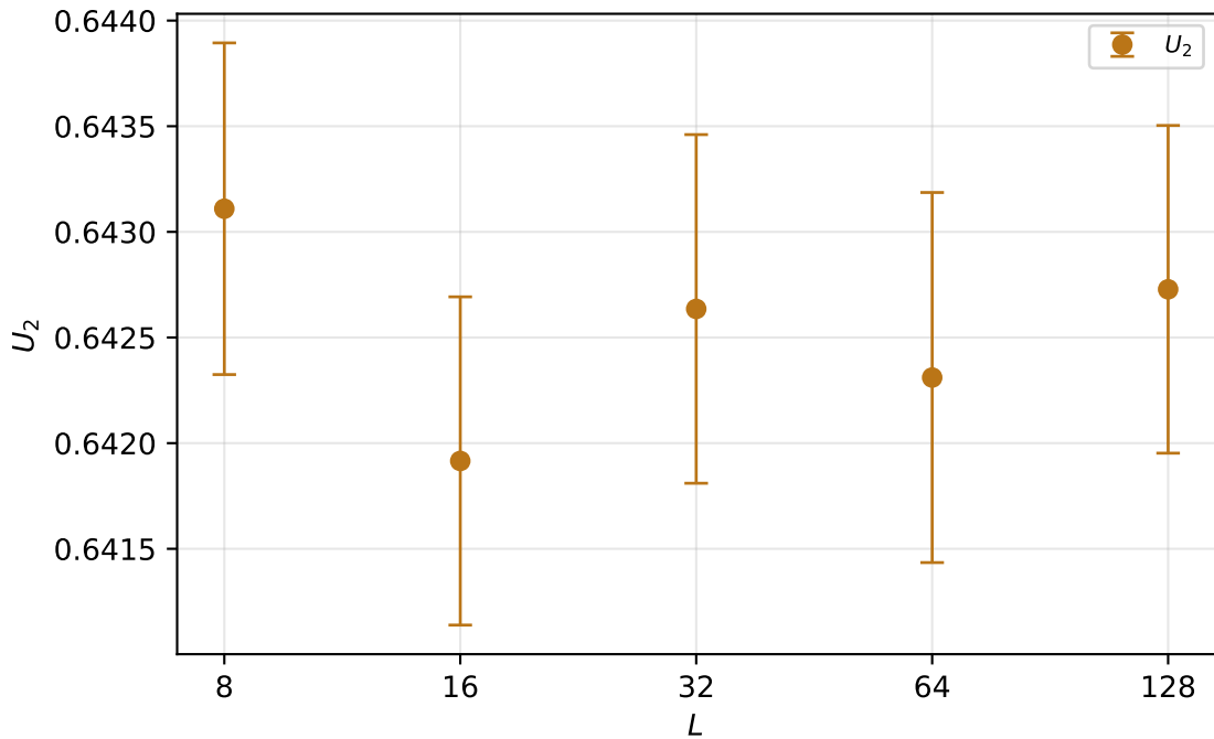
Binder cumulant U_2 vs L
