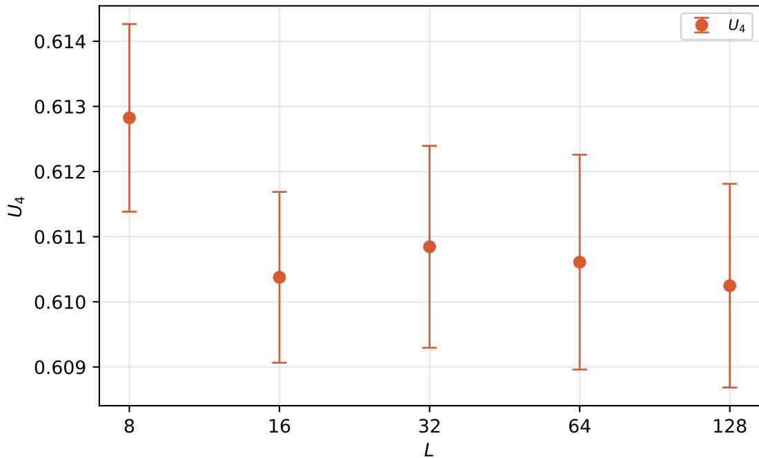
Binder cumulant U_4 vs L
