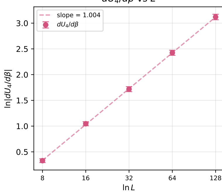
dU_4/d\beta vs L
