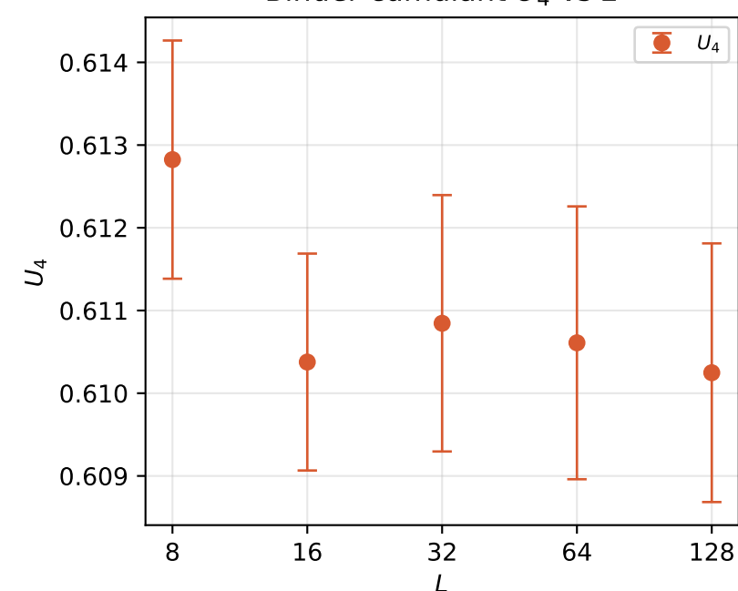
Binder cumulant U_4 vs L
