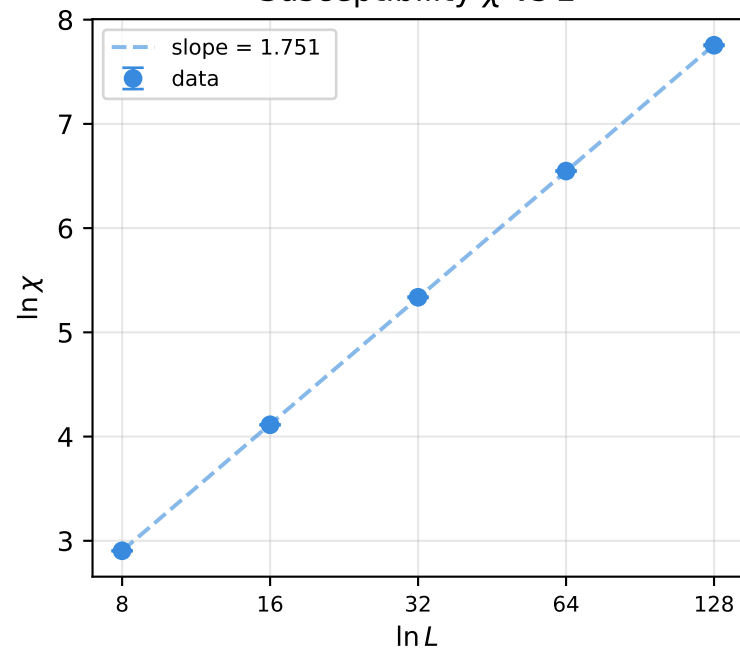
Susceptibility \chi vs L
