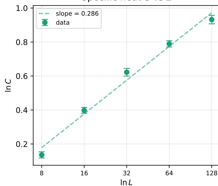
Specific heat C vs L
