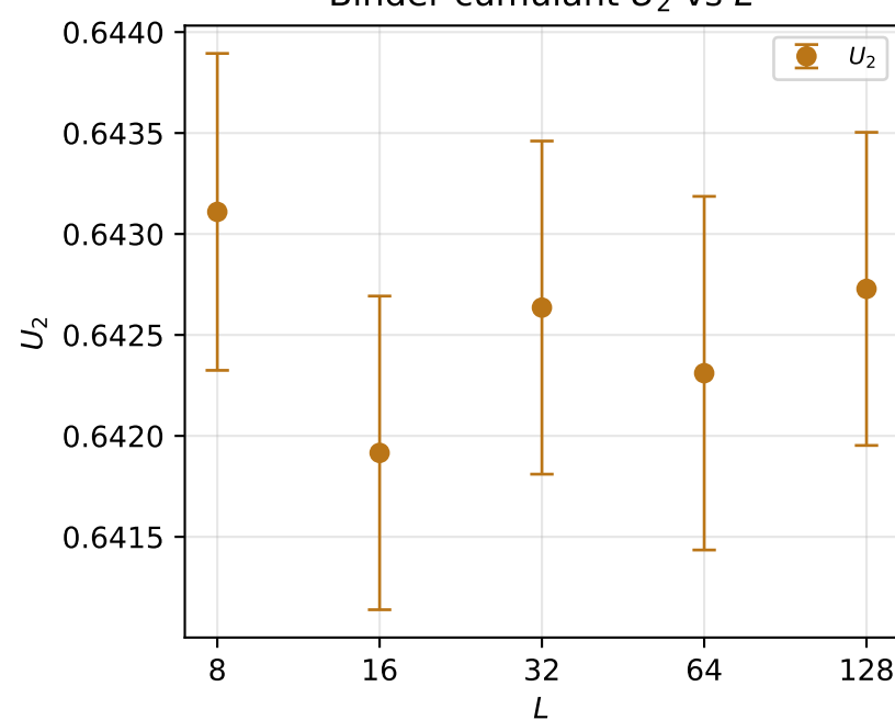
Binder cumulant U_2 vs L
