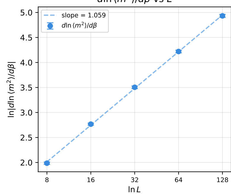
d \ln \langle m^2 \rangle / d\beta vs L
