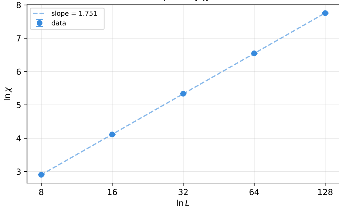
Susceptibility \chi vs L
