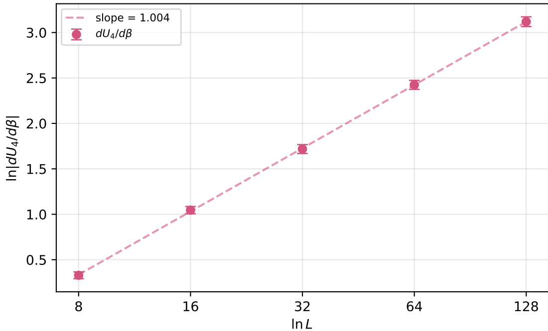
dU_4/d\beta vs L
