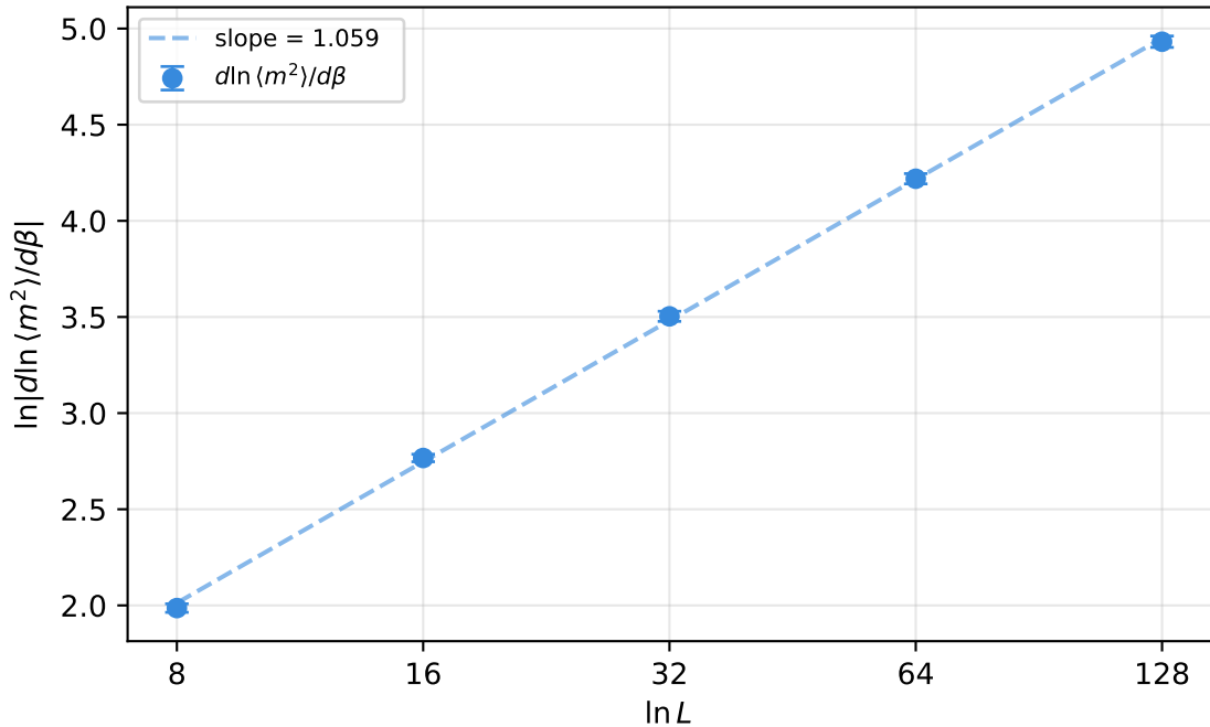
d\ln \langle m^2 \rangle / d\beta vs L
