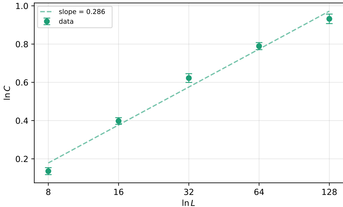
Specific heat C vs L
