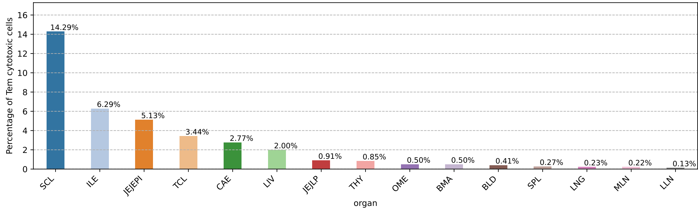
Percentage of SIGMA-identified Tem cytotoxic lymphocytes by organ
