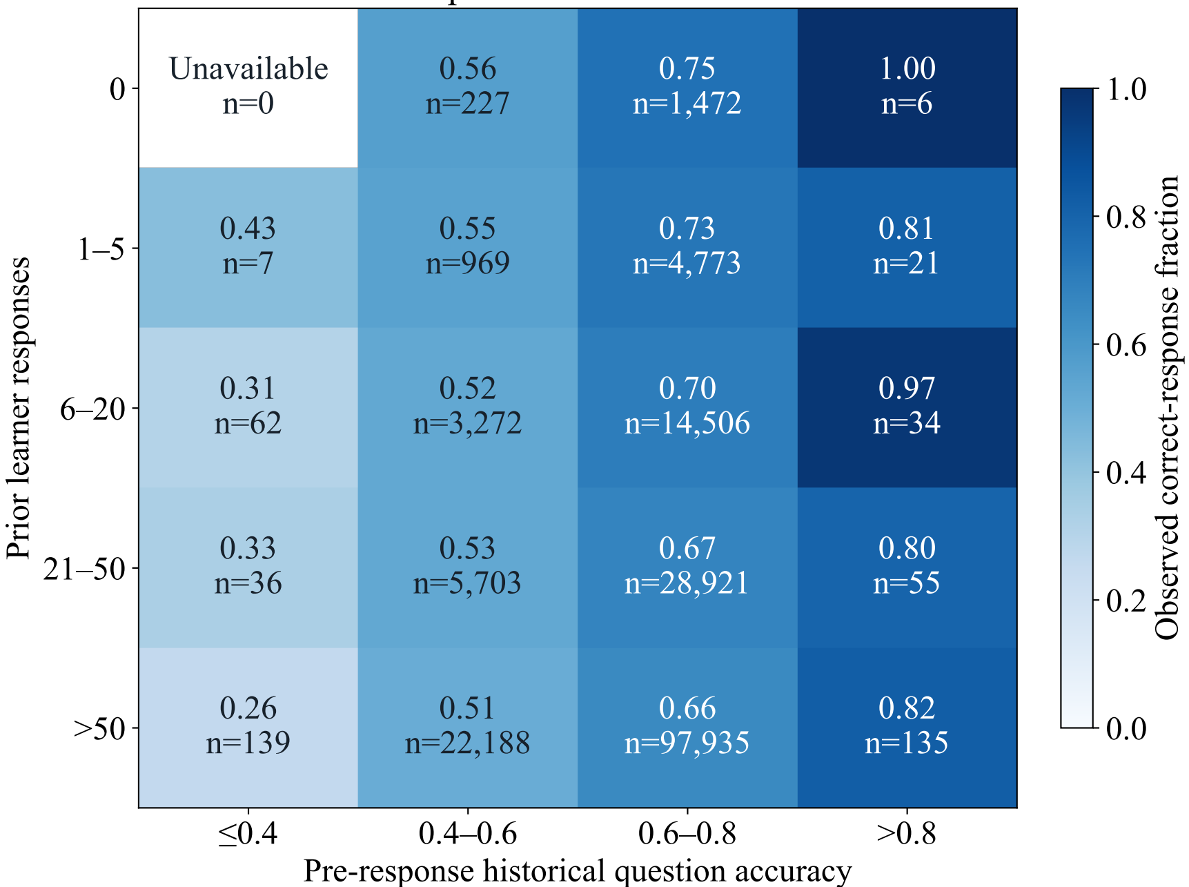
Development outcome structure
