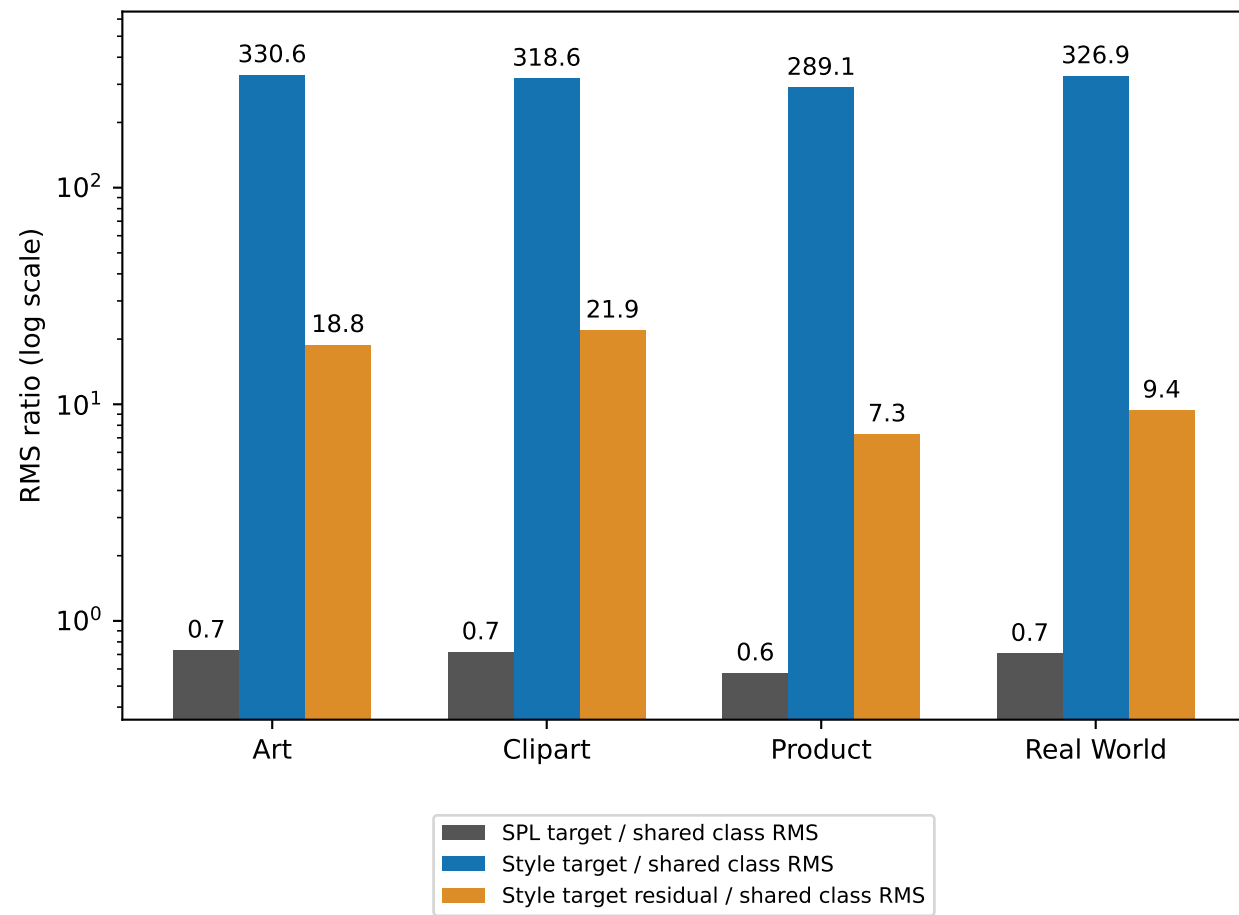
Domain vs shared CLASS context (16 tokens each)
