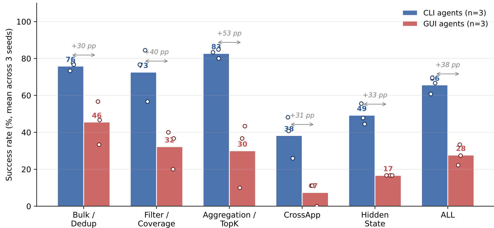
Tier-4 success rate by category — CLI vs GUI paradigm gap
