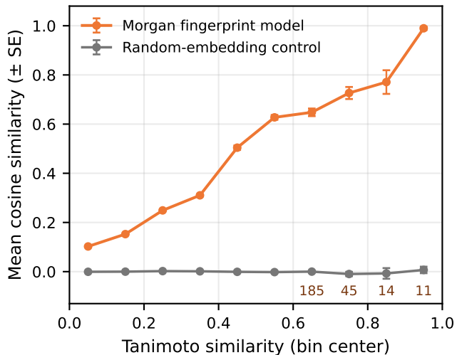
B. Mean by Tanimoto bin
