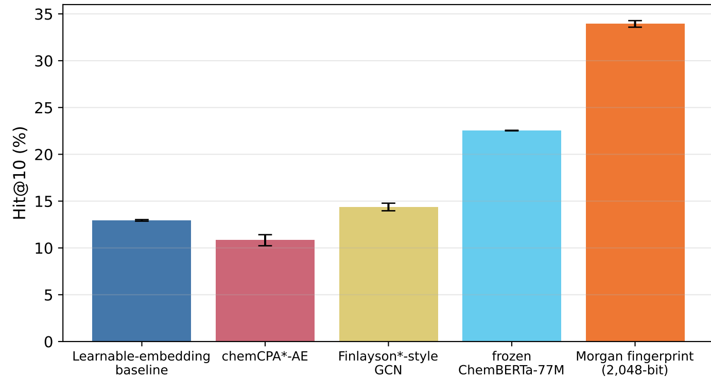
Hit@10 (3-seed mean \pm SE)
