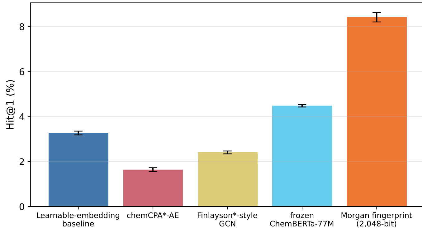
Hit@1 (3-seed mean \pm SE)
