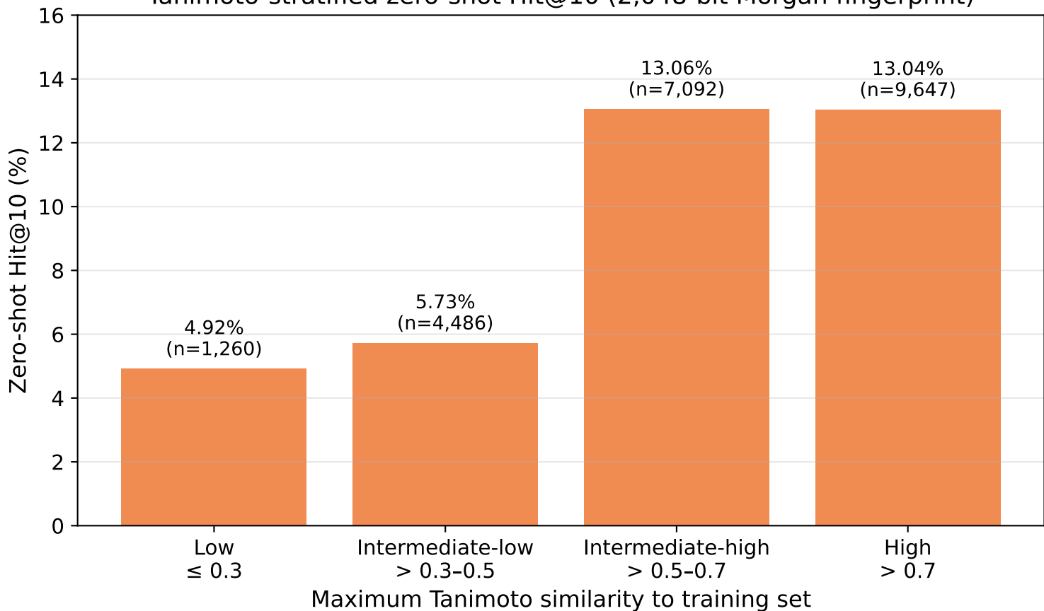
Tanimoto-stratified zero-shot Hit@10 (2,048-bit Morgan fingerprint)
