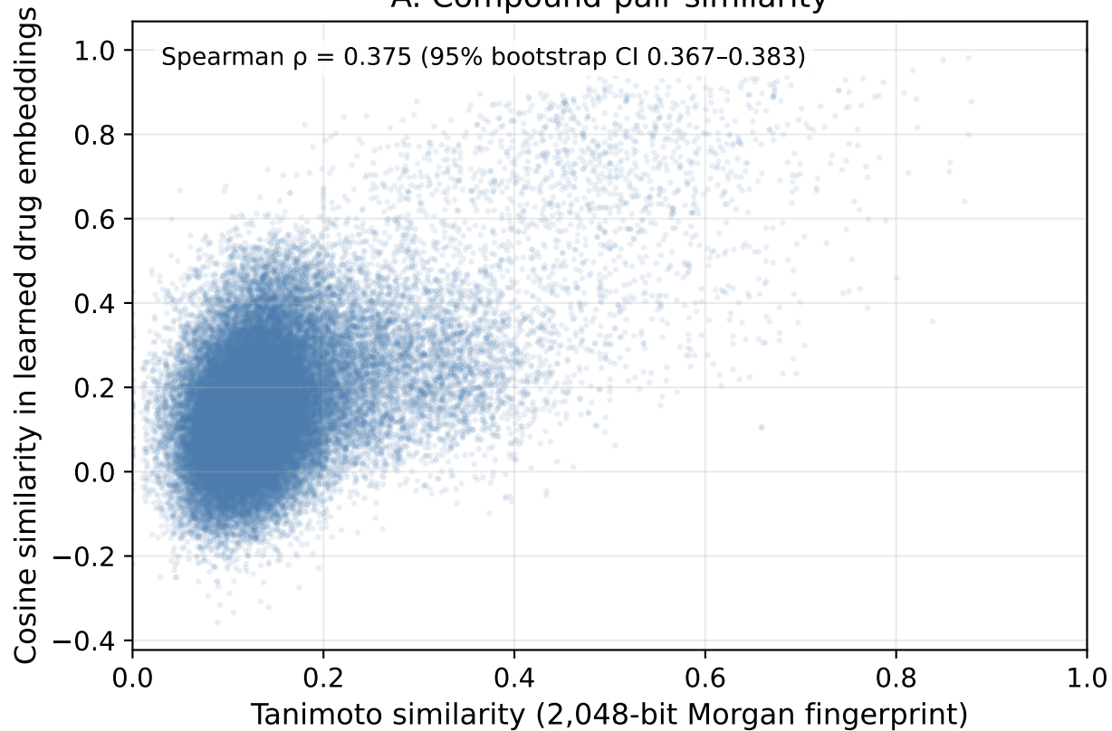
A. Compound-pair similarity
