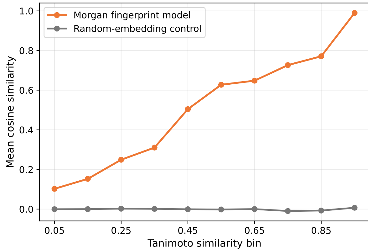
B. Mean embedding similarity by Tanimoto bin
