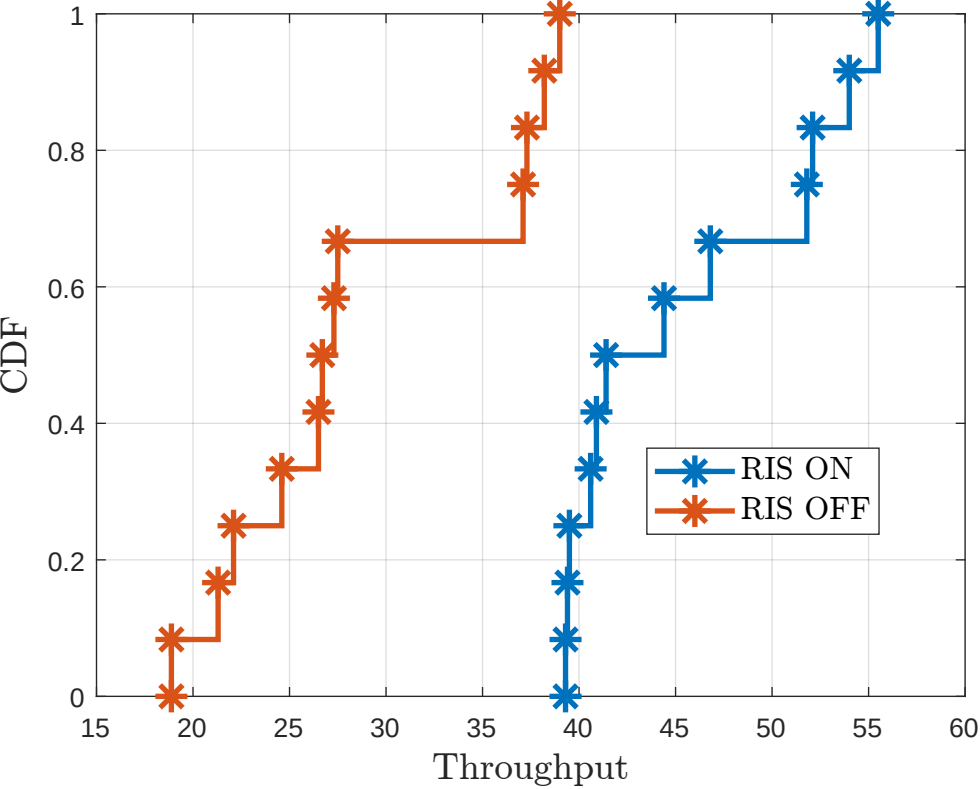
CDF of Throughputs: RIS ON vs RIS OFF
