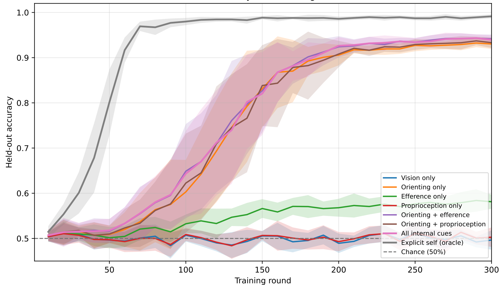
Cue ablations: held-out accuracy over training (mean \pm std, 10 seeds)
