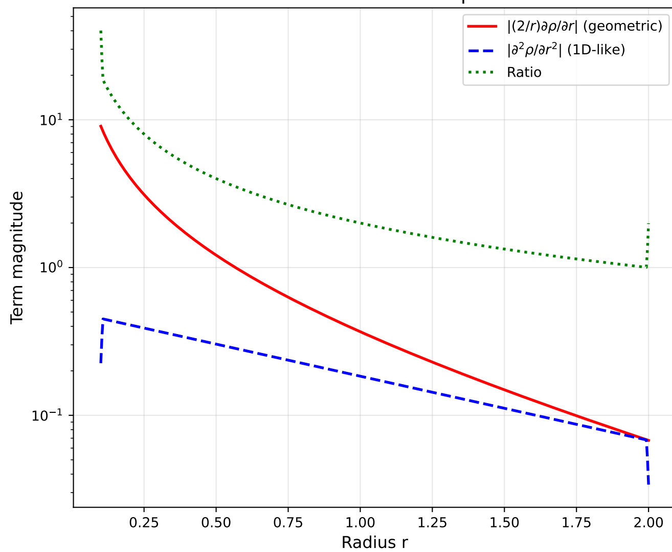
Geometric Term vs 1D Laplacian
