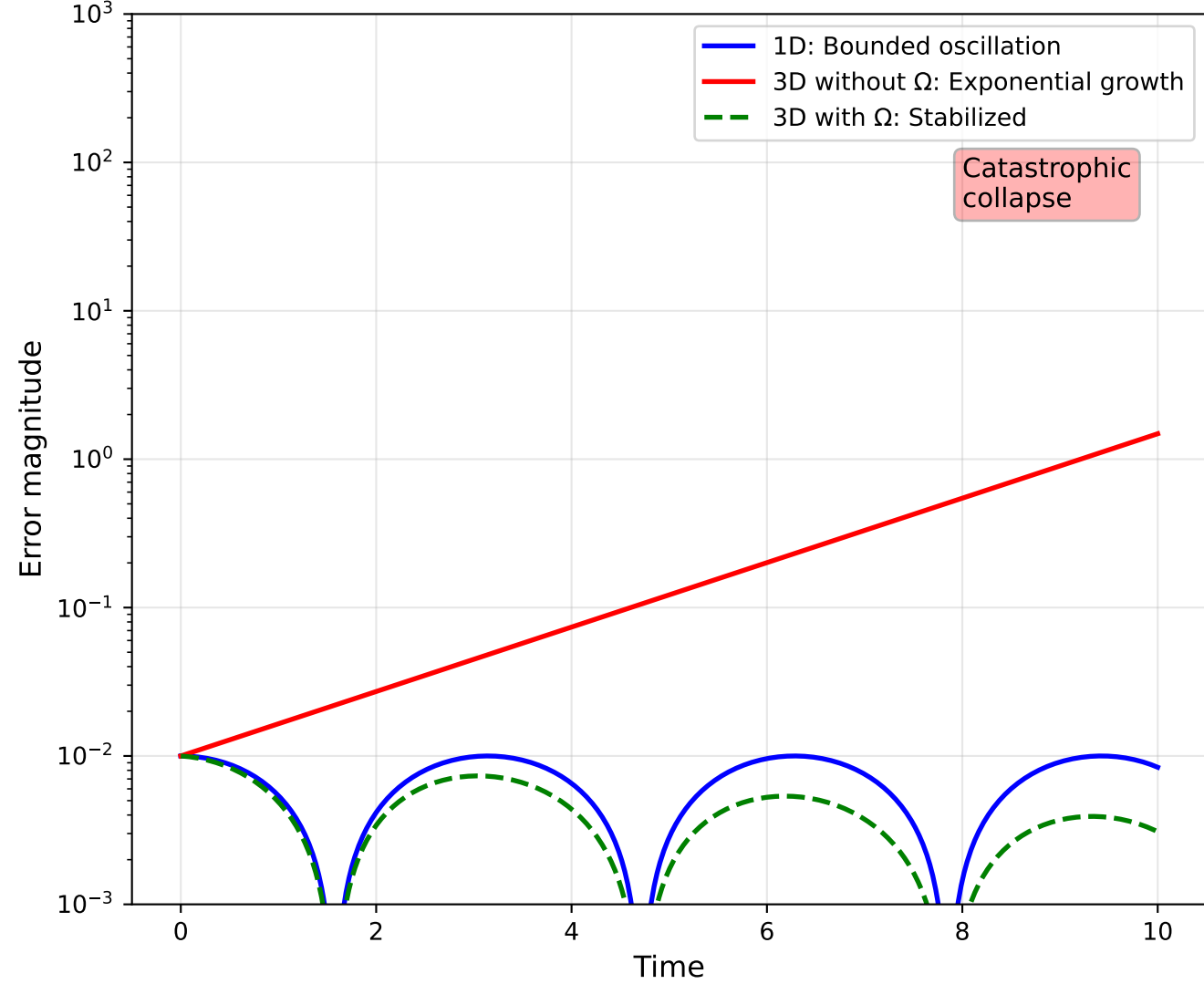
Error Evolution: 1D vs 3D
