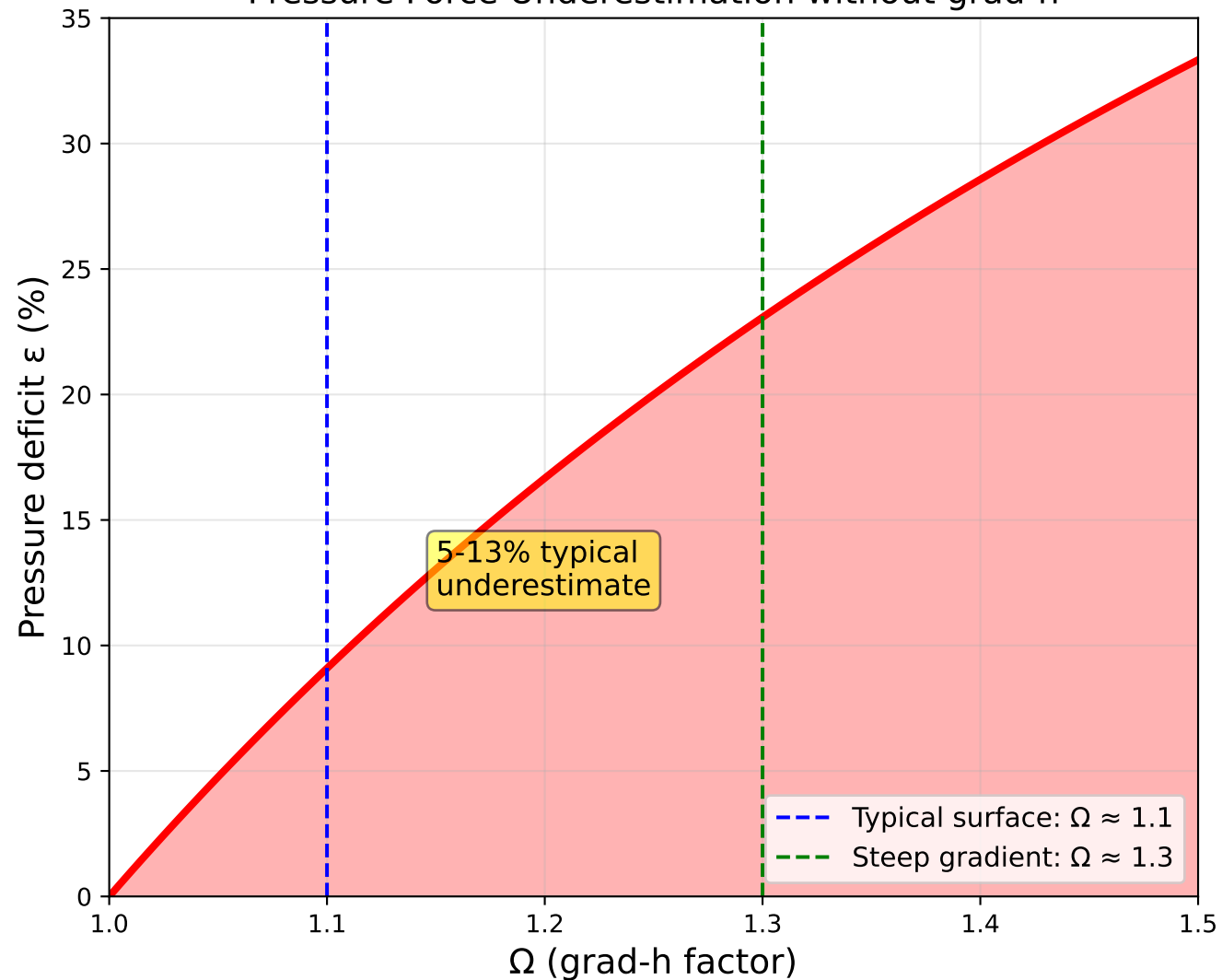
Pressure Force Underestimation without grad-h
