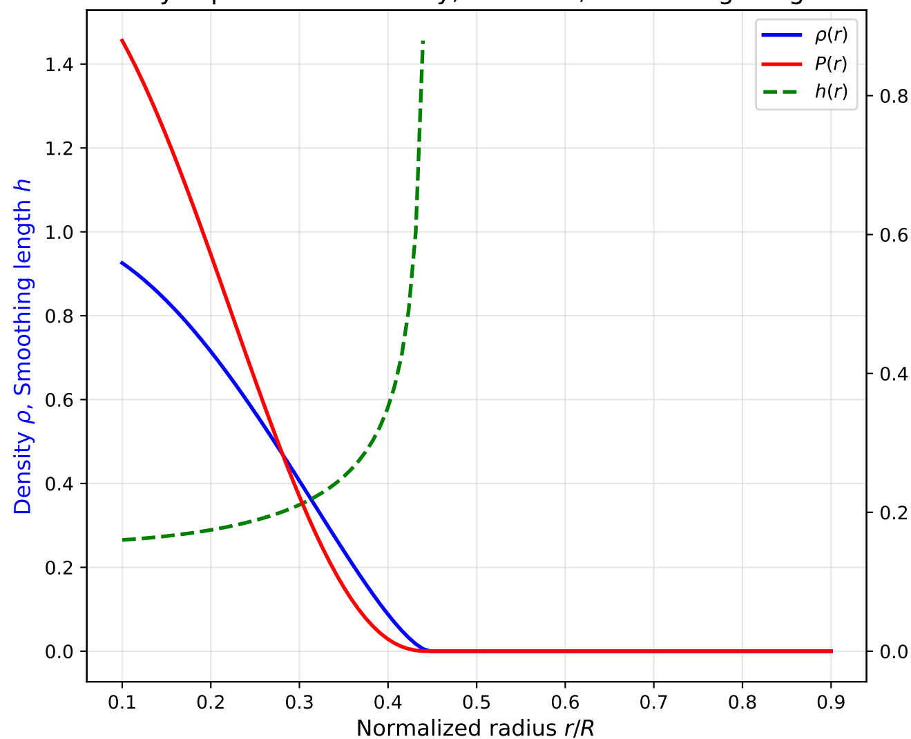
GSPH: Ratio Corrupted by Kernel Gradients
