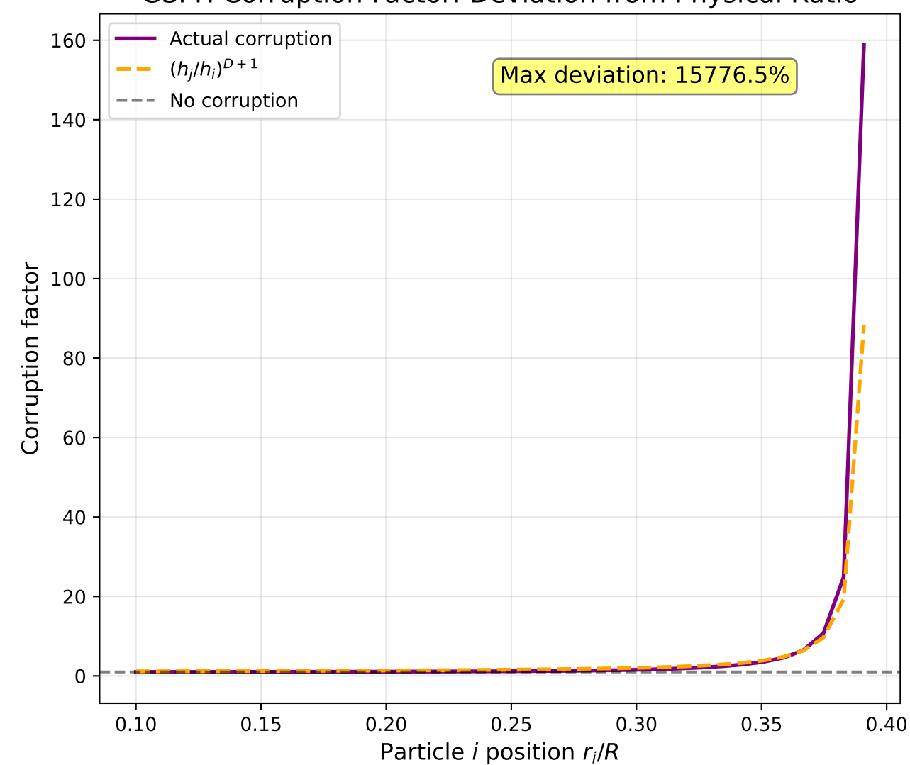
GSPH Corruption Factor: Deviation from Physical Ratio
