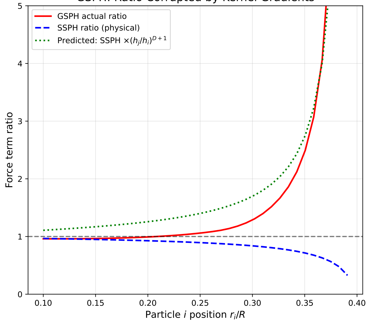
GSPH: Ratio Corrupted by Kernel Gradients
