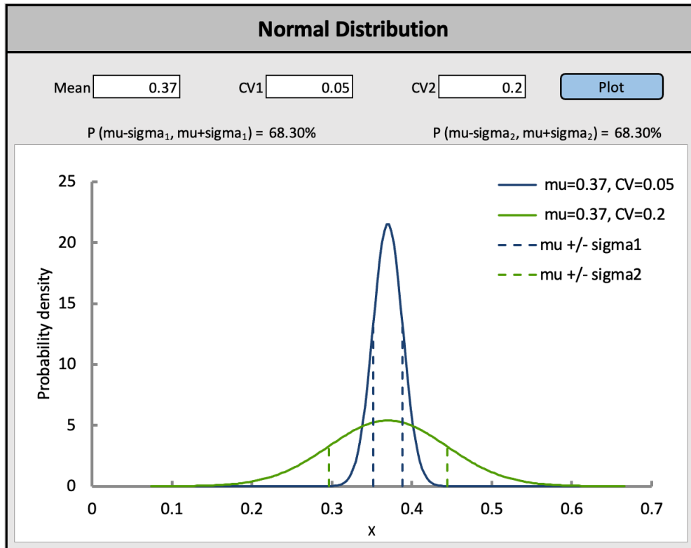
Figure 17: Visualization of the sampling distribution for \theta_s under a normal distribution.
