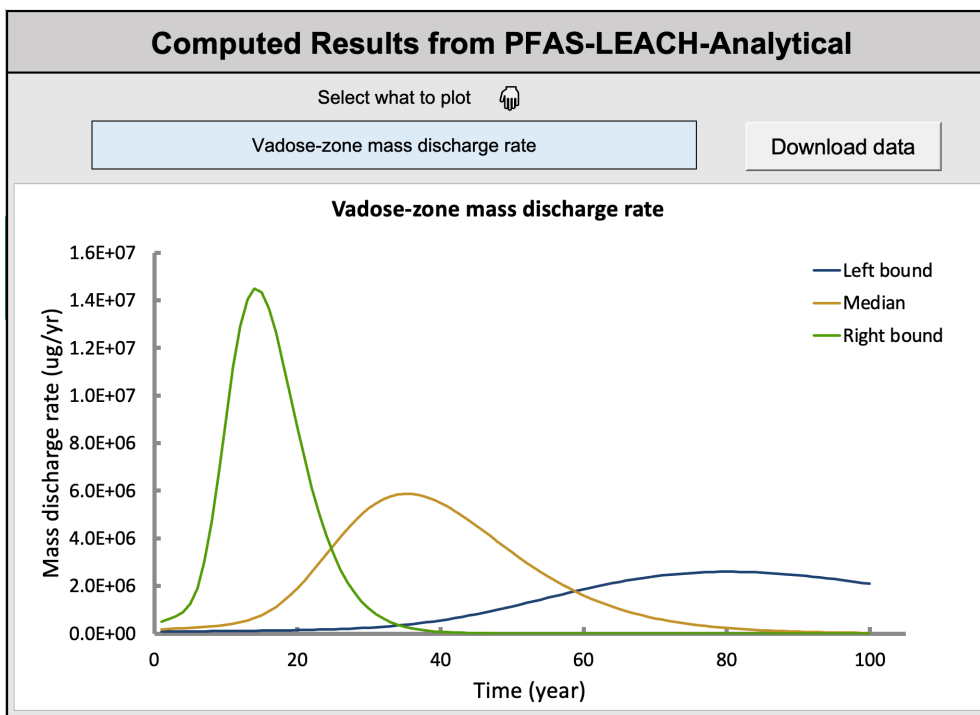
Figure 13: Module 1 output. Vadose-zone mass discharge rate computed from PFAS-LEACH-Analytical (basic solver). The three curves represent left-bound (blue), median (yellow), and right-bound (green) parameter sets.
