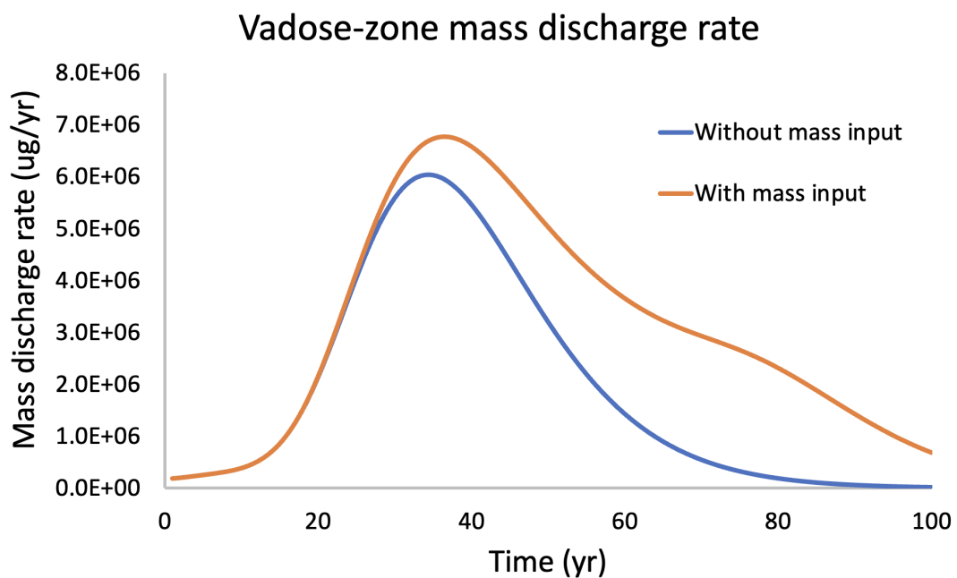
Figure 11: Module 0 output. Simulated vadose-zone mass discharge rate by PFAS-LEACH-Analytical with and without PFAS mass loading at the upper boundary. The upper boundary input scenario assumes a PFAS release period of 50 years and a release rate of 0.1 \mu\text{g}/\text{cm}^2/\text{year} .
