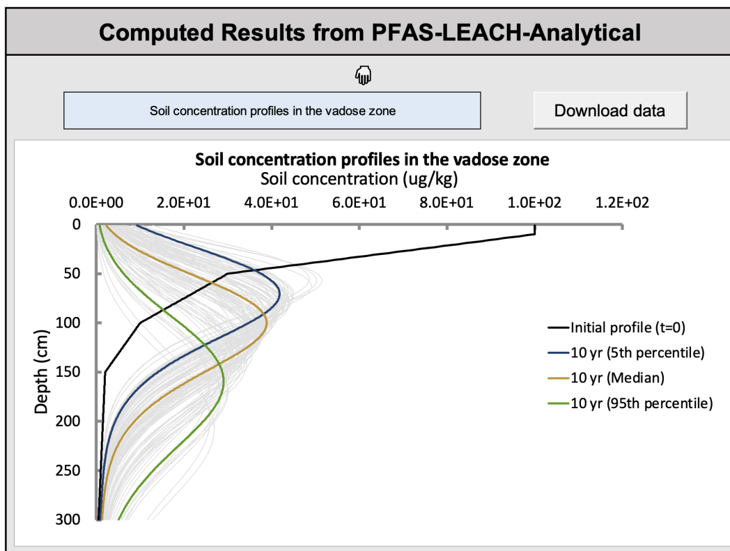
Figure 24: Module 2 output. Soil concentration profiles in the vadose zone computed with PFAS-LEACH-Analytical (basic solver). The black line indicates the initial profile ( t = 0 ). Gray lines represent individual Monte Carlo realizations after 10 years, while the blue, orange, and green lines show the 5 th percentile, median, and 95 th percentile profiles based on leaching risk ranking.
