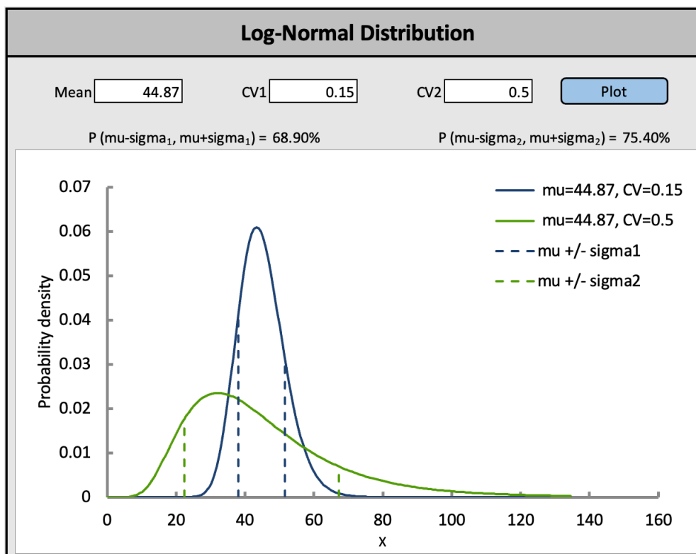
Figure 18: Visualization of the sampling distribution for K_s under a log-normal distribution.
