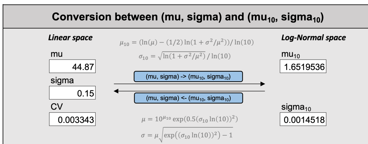
Figure 19: Conversion tool for translating parameter statistics between linear space and \log_{10} -normal spaces.
