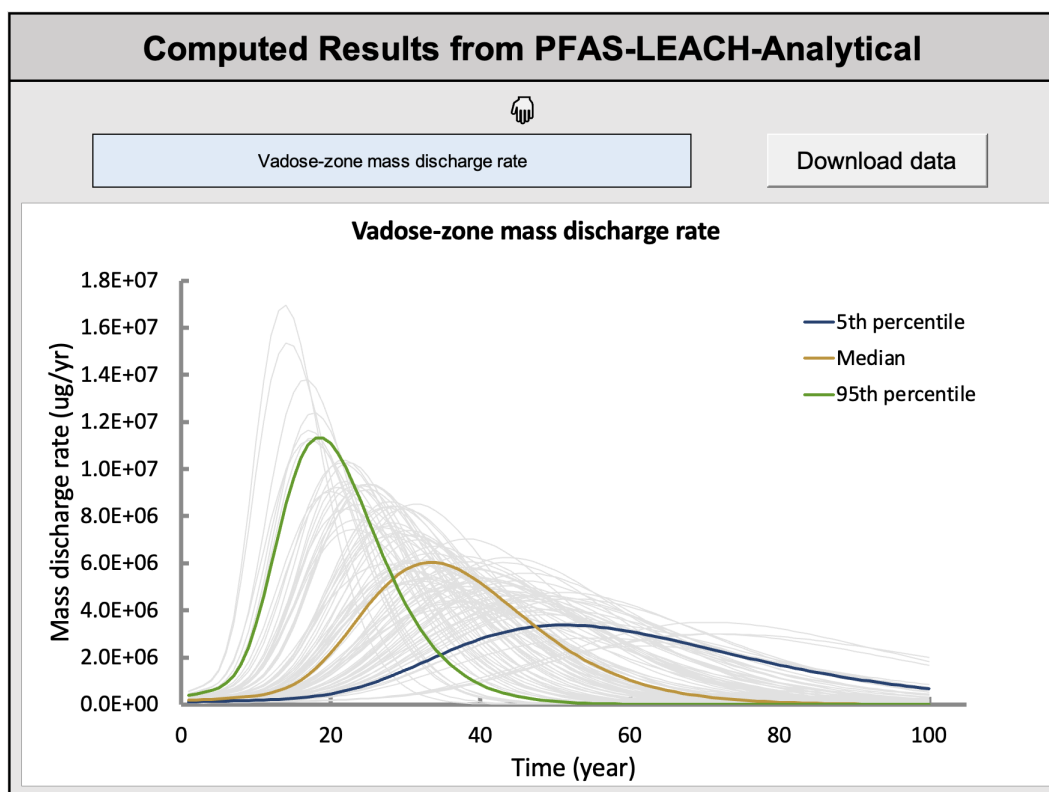
Figure 23: Module 2 output. Vadose-zone mass discharge rate computed with PFAS-LEACH-Analytical (basic solver). The gray lines represent individual Monte Carlo realizations, while the colored curves indicate the 5 th percentile, median, and 95 th percentile based on leaching risk ranking.
