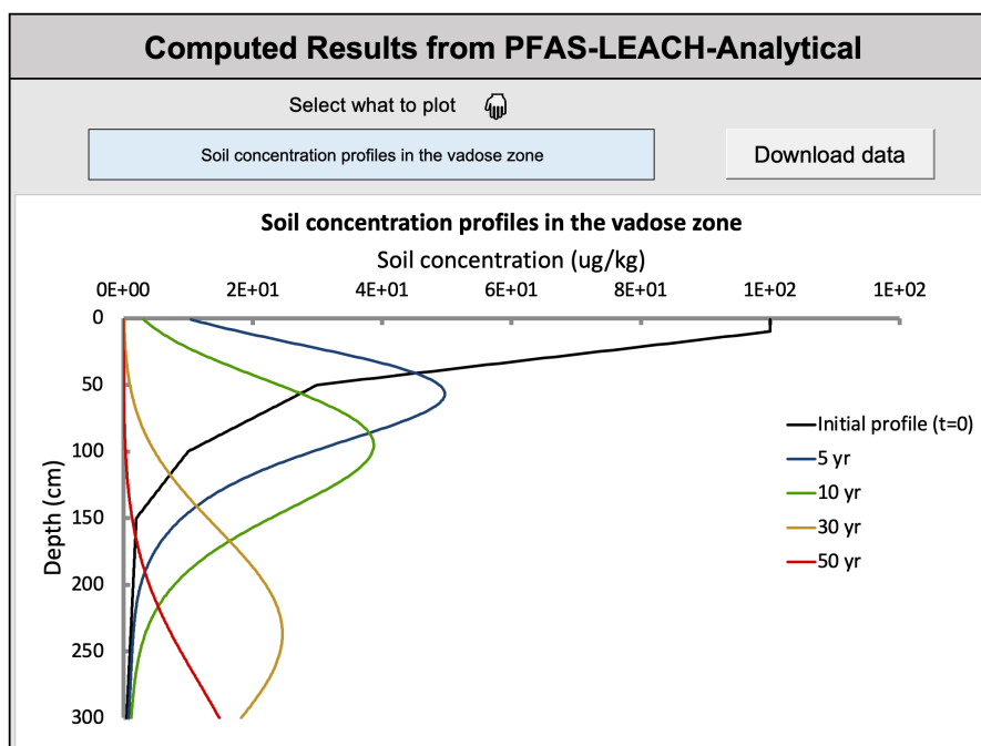
Figure 8: Module 0 output. PFAS soil concentration profiles at selected time points from PFAS-LEACH-Analytical (basic solver). Users can use the drop-down menu to also display PFAS aqueous concentration profiles in the vadose zone.
