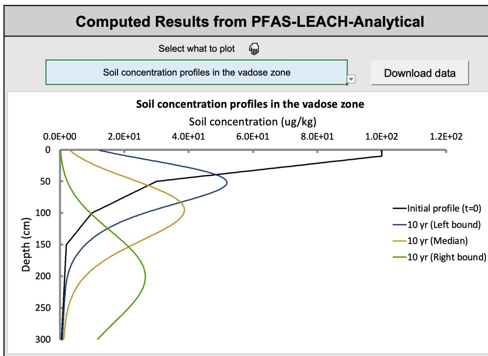
Figure 14: Module 1 output. Soil concentration profiles in the vadose zone after 10 years, computed from PFAS-LEACH-Analytical (basic solver). The three curves represent left-bound (blue), median (yellow), and right-bound (green) parameter sets.
