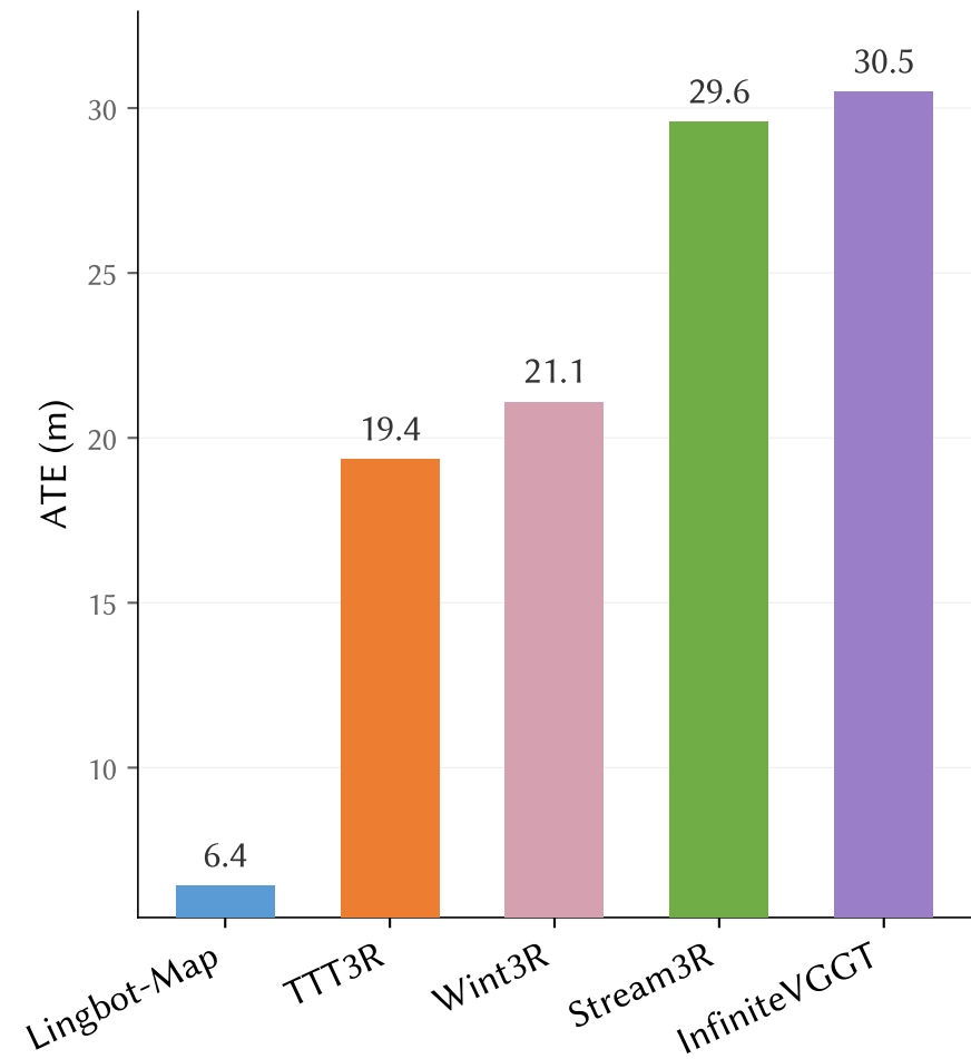
Oxford Spires ATE ↓
