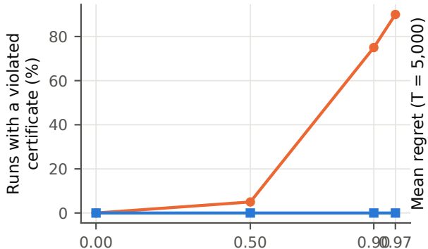
Standard certificates fail under persistence
