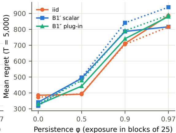
Valid certificates at comparable regret
