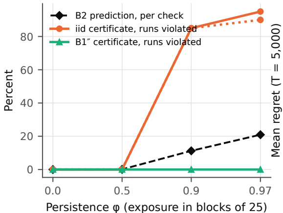
B2 predicts when iid certificates fail
