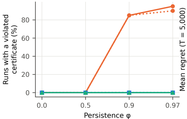
iid certificates fail as persistence grows
