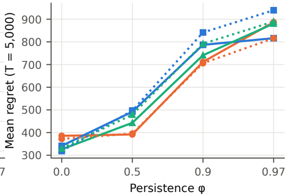
Valid certificates, comparable regret
