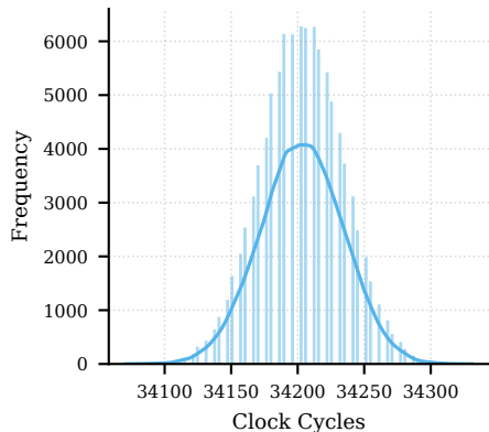
STM32 AES (S-box)
