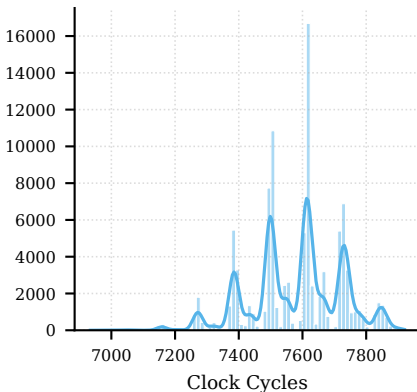
RP2350 AES (S-box)
