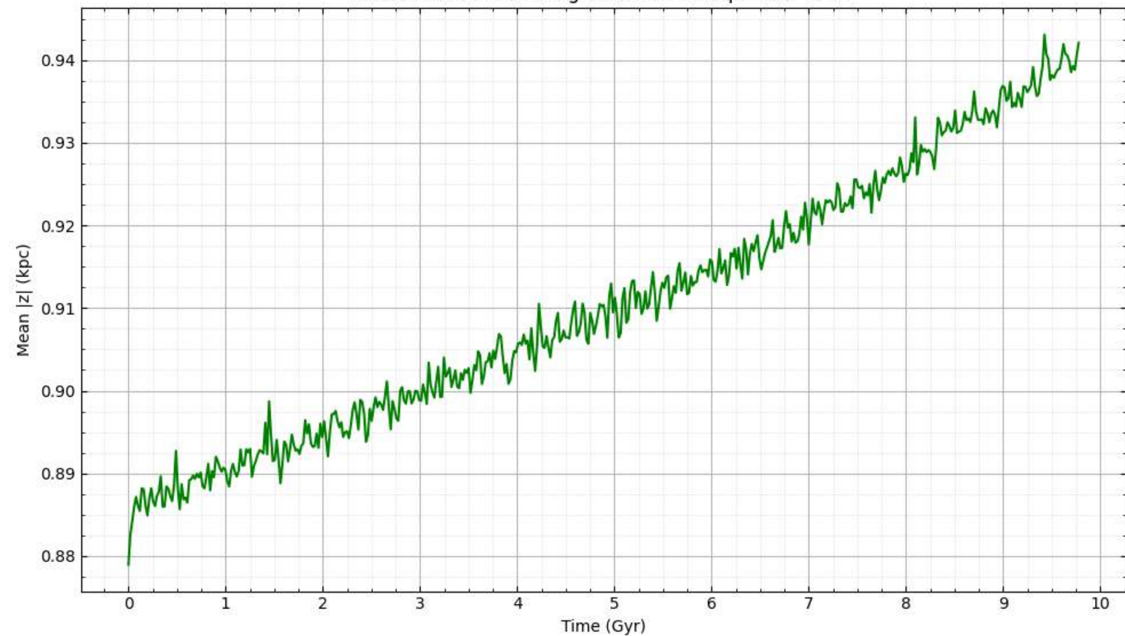
Disk Mean Vertical Height within 10.0 kpc over Time
