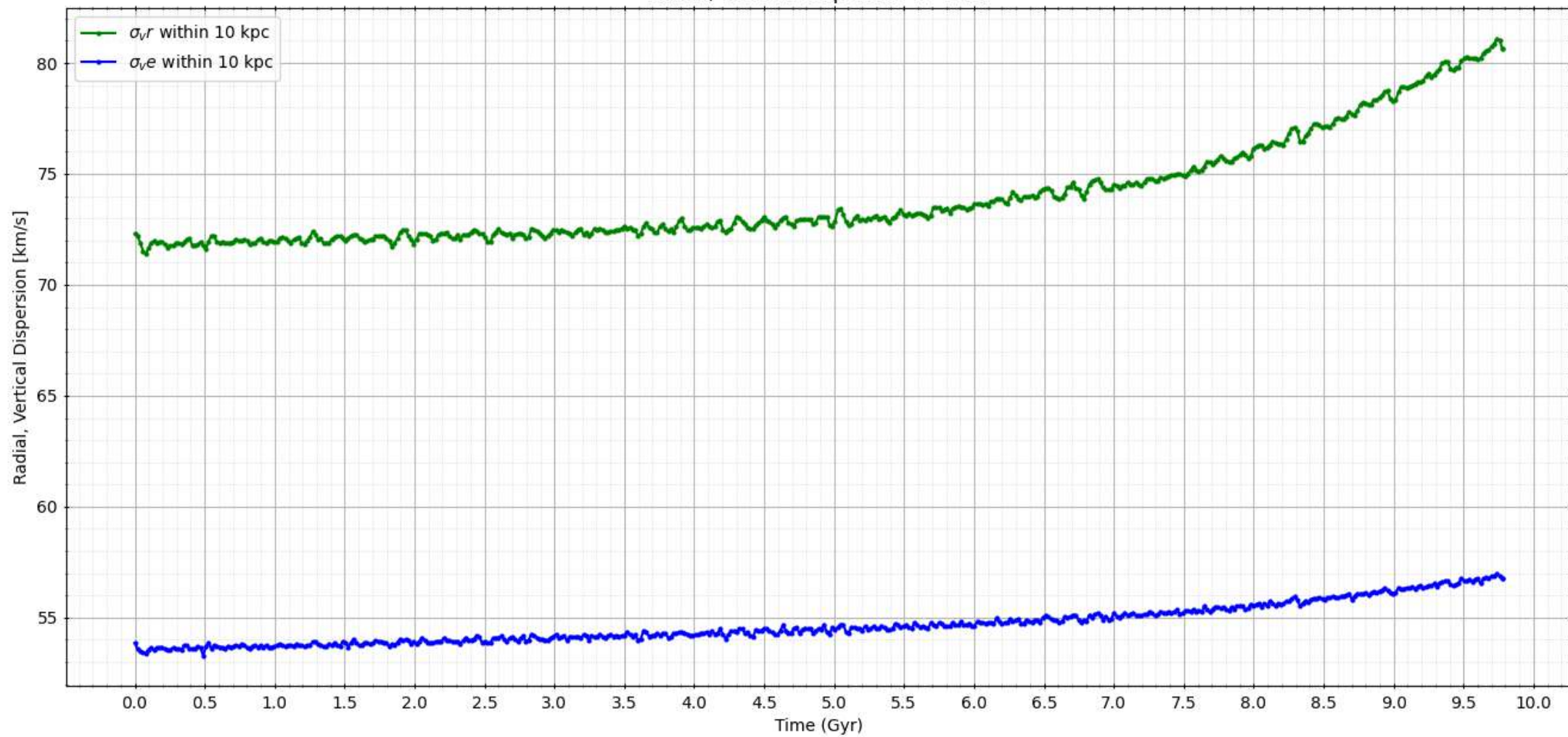
Radial, Vertical Dispersion vs Time
