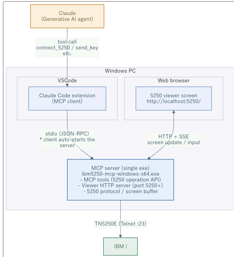
Figure 1.2-1 System Configuration (relationship among Claude / VSCode / browser / IBM i)
