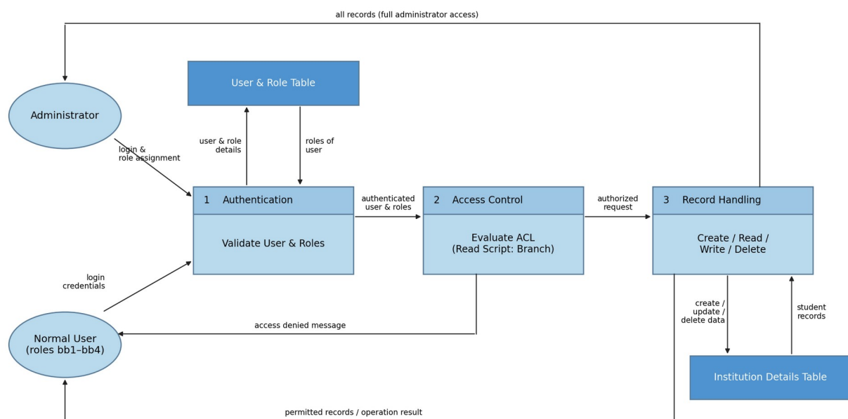
Data Flow Diagram – Script-Controlled ACL (Restrict Record Access Based on Field Value)
