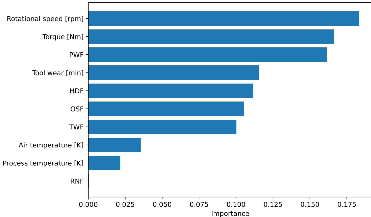
RQ1: Top 10 Feature Importances (RAW Sensor Fusion)
