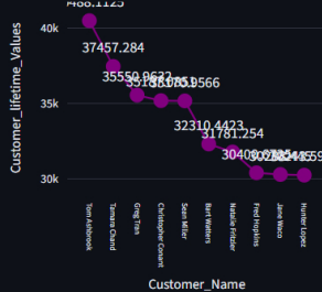
Customer_lifetime_Values Distributions
