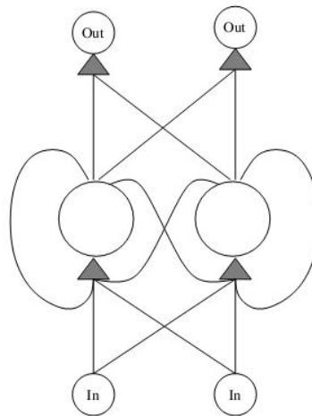
a simple RNN Elman
