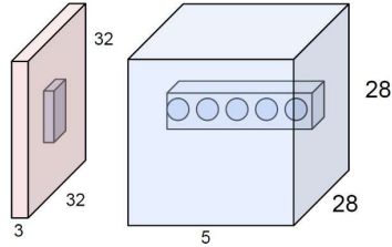
The brain/neuron view of CONV Layer
