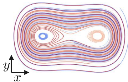
Duffing
