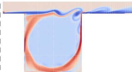
Cavity flow
