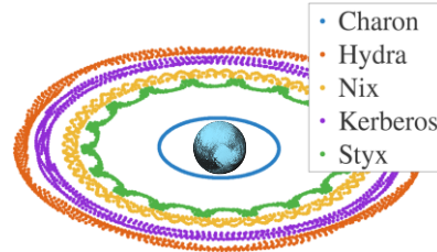
Pluto-Charon
