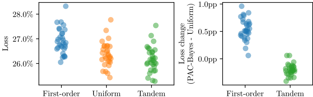
Voting ensembles, 30 members, CIFAR10
