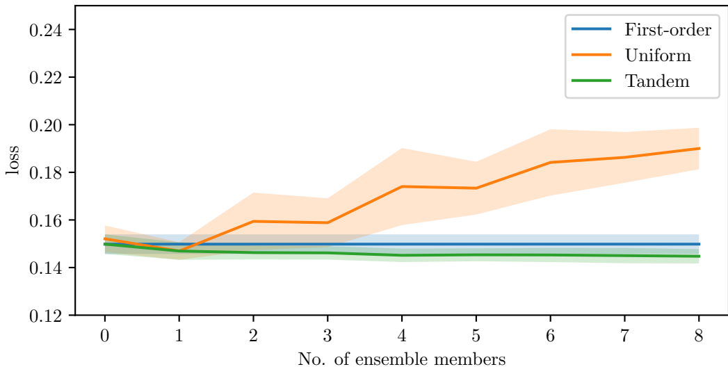
IMDB ensembles, bootstrapping ensemble members
