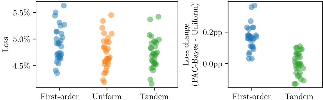
Voting ensembles, 15 members, CIFAR10
