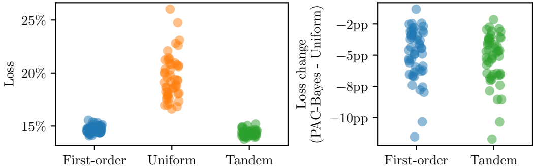
Voting ensembles, 10 members, IMDB
