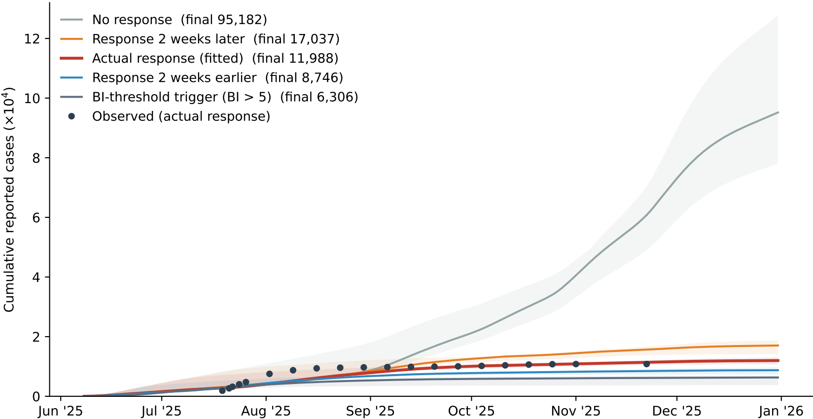
Fig. 3. Counterfactual reported-case trajectories under five response scenarios.
