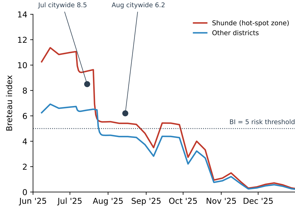
(b) Response-adjusted BI vs surveillance anchors
