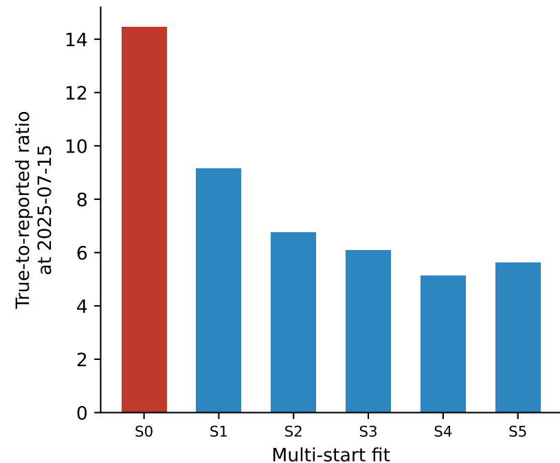
(a) Early under-ascertainment (multi-start envelope)
