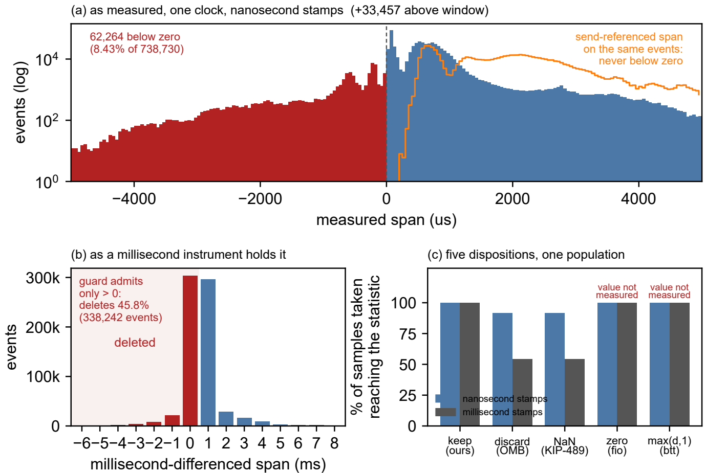
Fig. 6. What the instrument deletes, beside what it then reports. (a) At nanosecond resolution the acknowledgment-referenced span goes below zero 62,264 times in 738,730; the send-referenced span, same events and same clock, never does. (b) A millisecond instrument cannot see (a): it differences two truncated stamps, so a sub-millisecond flight lands on 0 or 1 by tick alignment alone, and a positivity guard then deletes 45.8% of the population uncounted. (c) The five dispositions found in shipping software (Section ), applied to that same population. Every count is emitted from the committed corpus by scripts/span_histogram.py .
