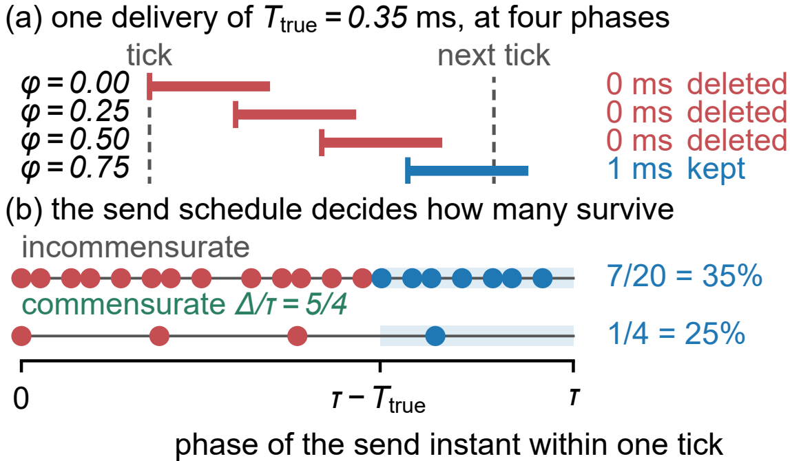
Fig. 10. Why a sample disappears, and why the survivors are not a sample. (a) One delivery of T_{\text{true}} = 0.35 ms at four phases of one tick. Three finish inside it, so both stamps round alike, the difference is exactly zero, and the guard removes them; the fourth crosses the boundary and is recorded as one whole tick — which is why the corpus prints 1.0 and 2.0 ms and nothing between. (b) A delivery survives from phase \tau - T_{\text{true}} onward — the shaded band — so uniform phases retain T_{\text{true}}/\tau (Equation 4); a commensurate producer visits only q and retains a count out of q , one of the values Equation 5 allows. T_{\text{true}} here is illustrative and off-vertex by choice: at 0.5 ms the two answers coincide.
