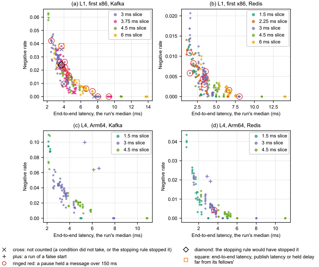
Fig. S17. Every slice run, aberrant runs marked. Each run of L1 (first x86 pair) and L4 (Arm pair, Arm64 in the panels) at its median end-to-end latency and its negative-span rate, colored by the slice it ran at. Crosses: runs the integrity rule did not count. Plusses: runs of L4's two false starts. Rings: counted runs with a warning, each reason its own shape (Table S32).
