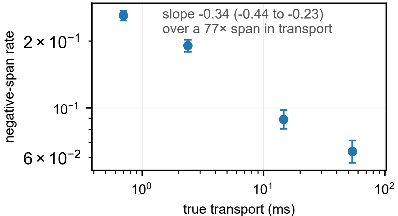
Fig. 6. A longer flight inverts less often. Negative span rate against true transport over the payload sweep, Wilson 95% intervals. The same stall distribution overlaps a short flight almost entirely and a long one hardly at all, which is Equation 3 of the main text as an experiment: lengthening what is being measured lowers the rate, where a load-driven account predicts no change. The figure sits here rather than in the main text for the same reason Equation 2 does — it draws four points.
