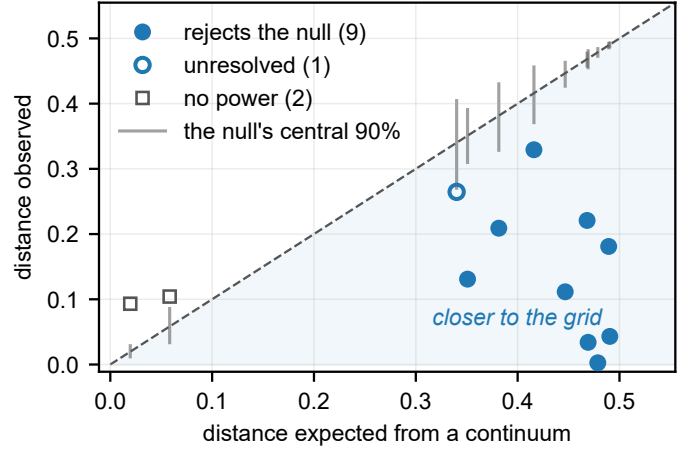
Fig. 4. Grid membership, as a set . Each arm's observed mean distance to the nearest grid vertex against the distance a continuum would give, which is the diagonal. The gray bar at each arm is that arm's own null, simulated: a marker clear of its bar is an arm that rejects, so the picture carries the test rather than illustrating it. Filled circles reject after Holm correction; the open circle is the one powered arm that does not, and it sits at the edge of its bar rather than clear of it. The 2 squares are the arms where the two hypotheses coincide and no test has power; their bars collapse towards zero, which is what having no power looks like, and the sign carries nothing there. Per-arm corrected p -values are in Supplement S46.
