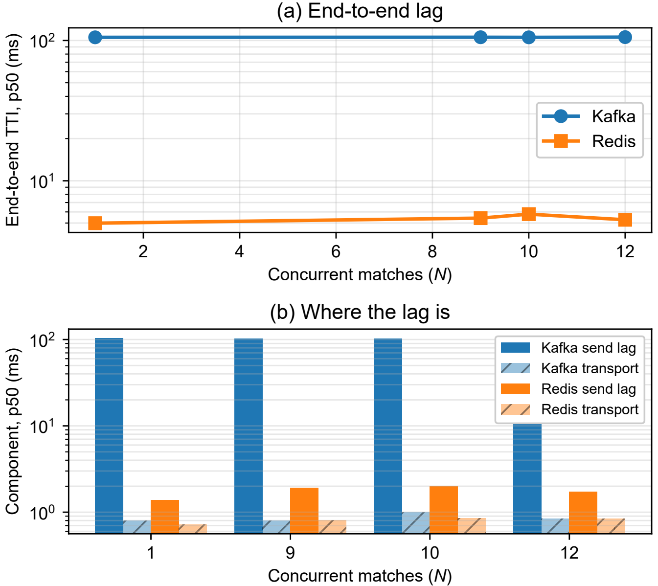
Fig. 2. Withdrawn. (a) End-to-end delay against concurrency as originally measured. (b) The decomposition that appeared to place the whole gap in producer send lag. Both panels are retained as evidence for the main text: the runs behind them matched a median of seven events each, so the apparent per-event offset is a per-run start-up cost. Broker transport, the lower series in (b), is unaffected and is what the paper claims.
