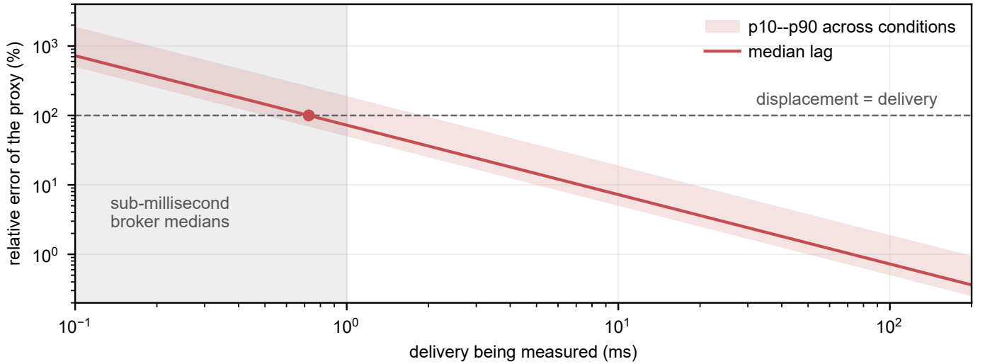
Fig. 8. Where a path sits on the exposure curve. Table XXIII as a curve: the relative error of the acknowledgment-referenced proxy, A/T_{\text{true}} , against the delivery being measured. The line is this corpus’s median acknowledgment lag and the band its tenth to ninetyth percentile across conditions, so a reader can bracket their own path rather than take the middle. The marked point is the crossover at 0.72\ \text{ms} , where the displacement equals the delivery it is a correction to; to its left the correction is larger than the quantity corrected. The shaded column is where published broker medians sit ( \$52.3 ), which is the reason the curve matters.
