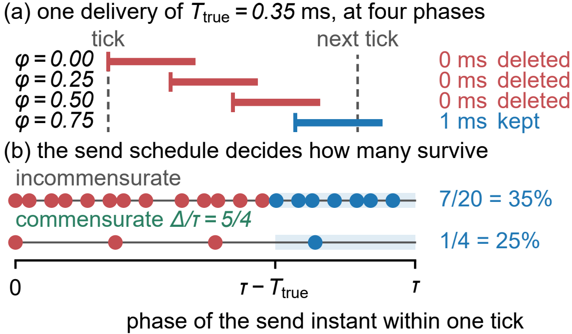
Fig. 12. Why a sample disappears, and why the survivors are not a sample. (a) One delivery of T_{\text{true}} = 0.35 ms at four phases of one tick. Three finish inside it, so both timestamps round alike, the difference is exactly zero, and the admission condition removes them; the fourth crosses the boundary and is recorded as one whole tick — which is why the corpus prints 1.0 and 2.0 ms and nothing between. (b) A delivery survives from phase \tau - T_{\text{true}} onward — the shaded band — so uniform phases retain T_{\text{true}}/\tau (Equation 4); a commensurate producer visits only q and retains a count out of q , one of the values Equation 5 allows. T_{\text{true}} here is illustrative and off-vertex by choice: at 0.5 ms the two answers coincide.
