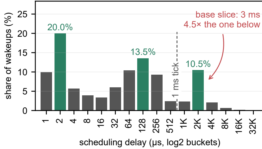
Fig. S4. Traced scheduling delays are trimodal. 551,956 wakeups, bpfttrace \log_2 buckets, modes shaded. The jitter peaks in the 2–4 \mu\text{s} bucket, which alone holds 20.0% of all wakeups. A second mode at 128–256 \mu\text{s} holds 13.5%. The third, at 10.5%, sits in the bucket holding the scheduler’s derived base slice of 3 ms. The count of modes survives a 2\times widening of the buckets in both phasings.
