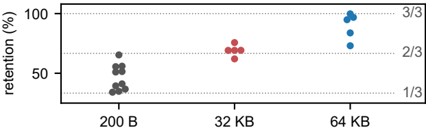
(a) Replicates against the q = 3 grid
